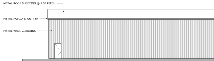
SOUTHERN ELEVATION
